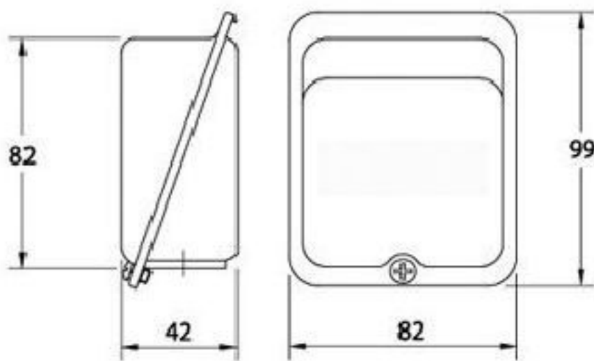
铁壳接线盒/Steel Plate Terminal Box
