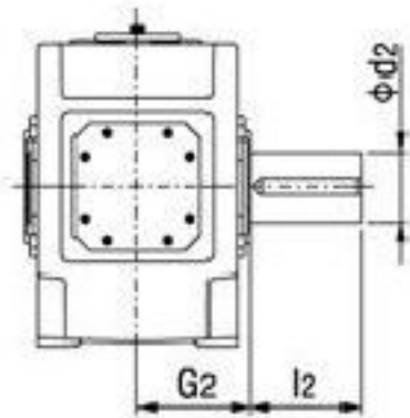
H2SH 实心轴 Solid shaft
