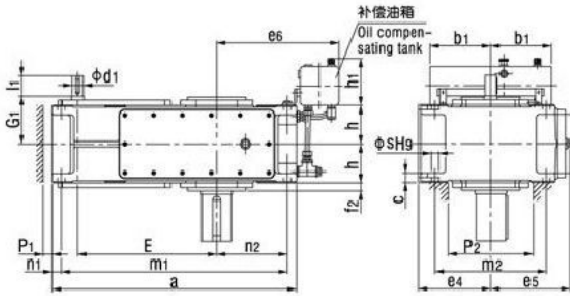
H3SV、H3HV、H3DV (浸油润滑 With dip lubrication)
