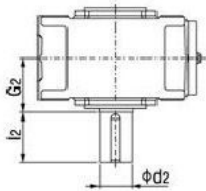
H3SV 实心轴 Solid shaft
