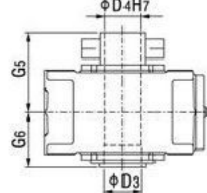
H3DV 带胀紧套的空心轴 Hollow shaft for shrink disk
