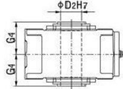
H3HV 空心轴 Hollow shaft
